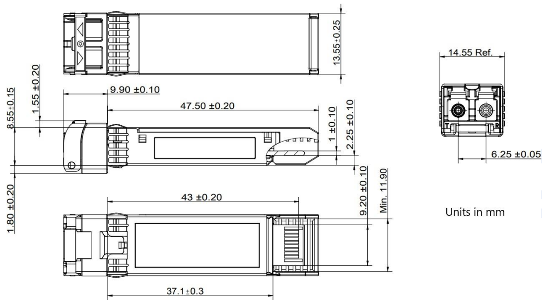
Figure2. Mechanical dimension
