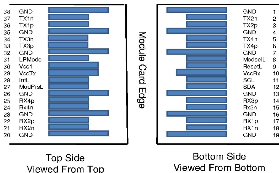
Figure 2, Pin View
