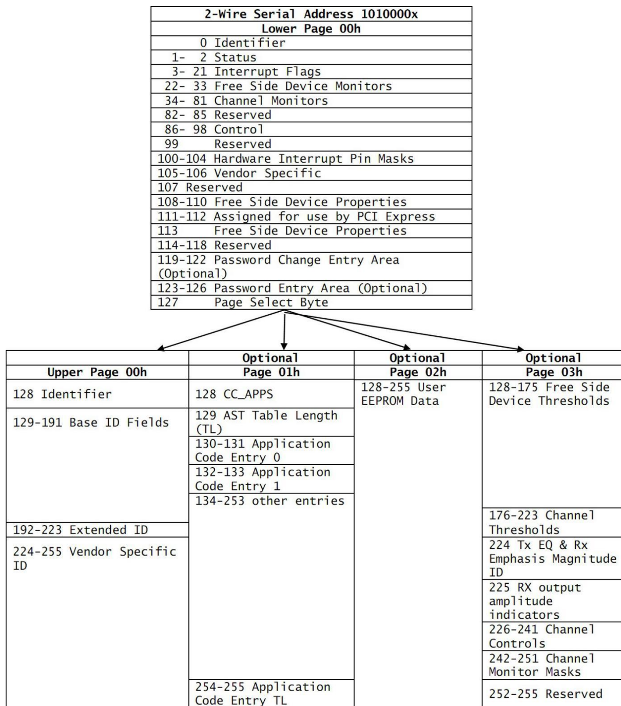
Figure 4, Memory Map
