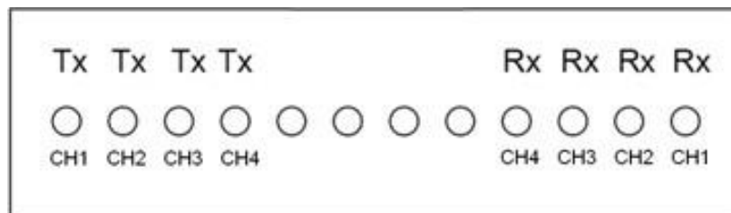
Figure 4, Optical interface arrangement. Lens upwards.
